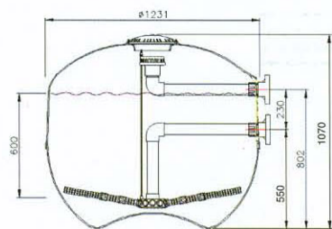
Laminated Filter 31115
