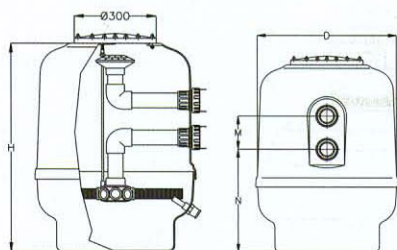
Laminated Filter Dimensions
